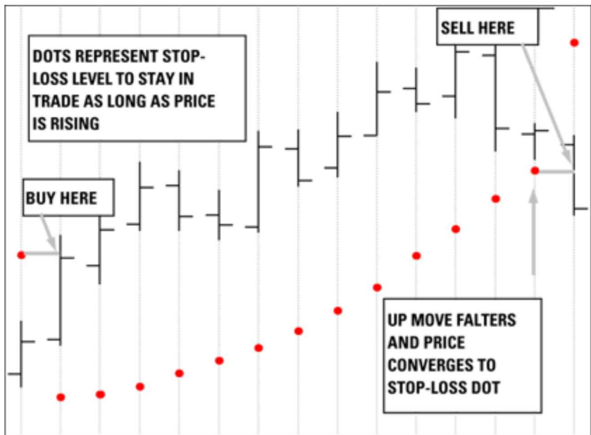
Figure 5-1: Parabolic stop.
