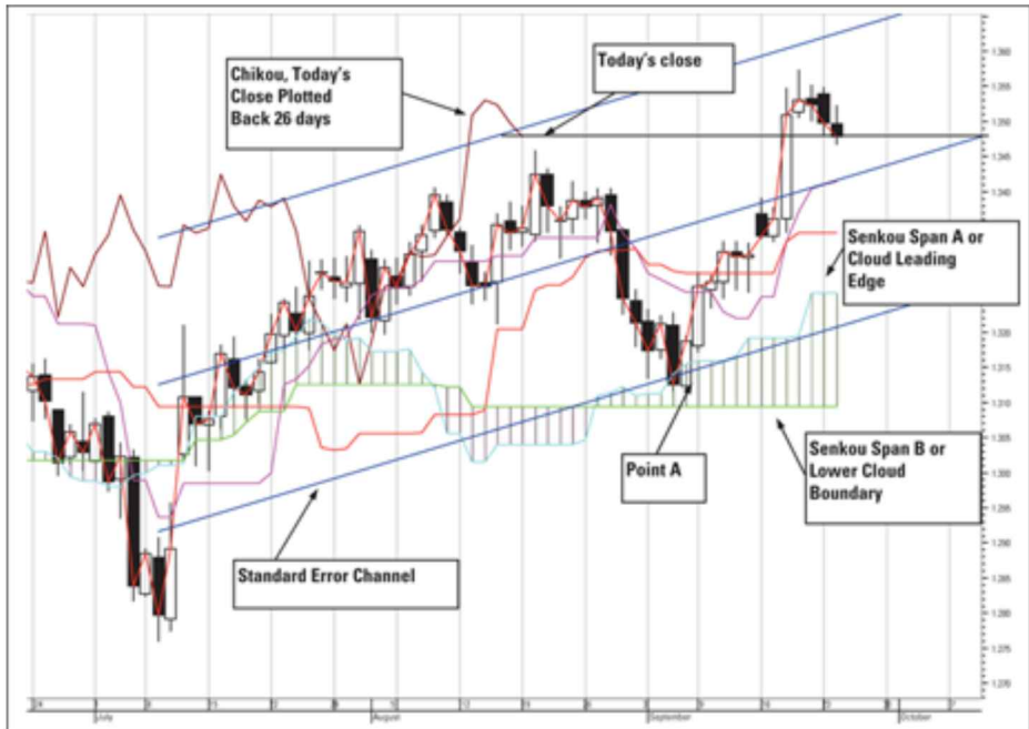
Figure 16-4: Ichimoku with the Standard Error Channel.
