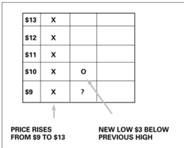
Figure 15-1: Point-and-figure chart format.
