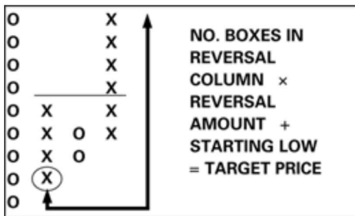
Figure 15-3: Vertical projection.
