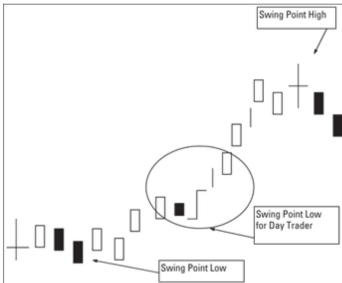
Figure 11-1: Swing points depend on timeframe.
