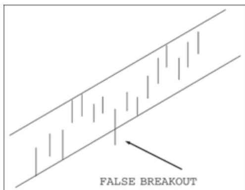
Figure 11-3: False breakout.
