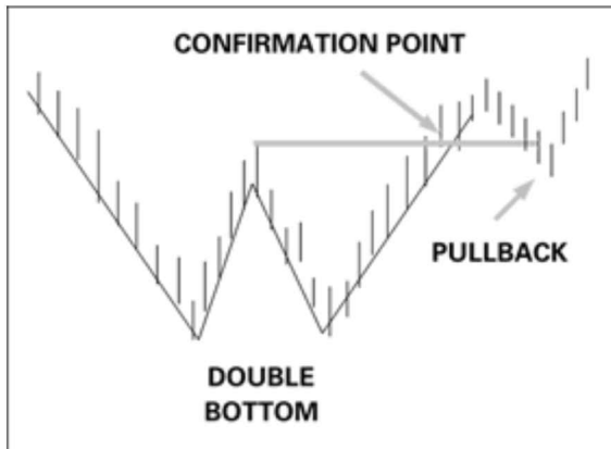
Figure 9-5: Double bottom.
