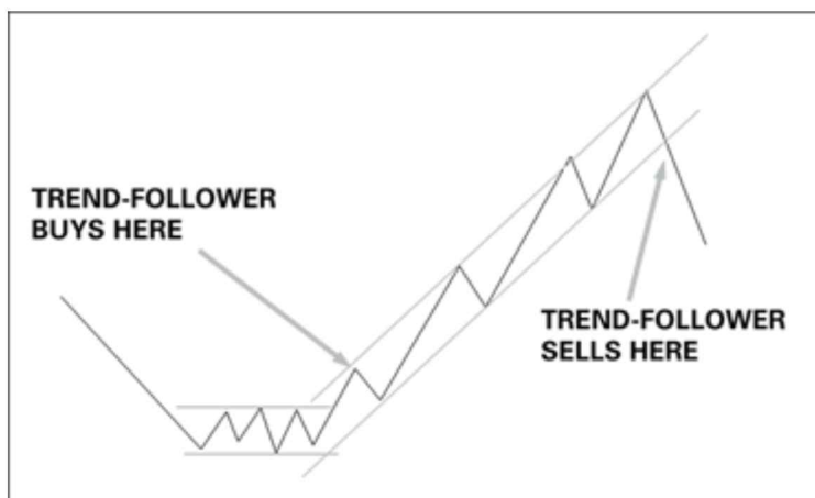
Figure 4-1: Trend-following.
