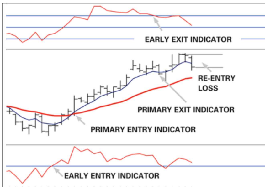
Figure 16-2: Confirming indicators.
