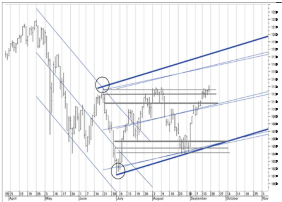
Figure 11-8: Pivot point levels overlaid with a standard error channel.
