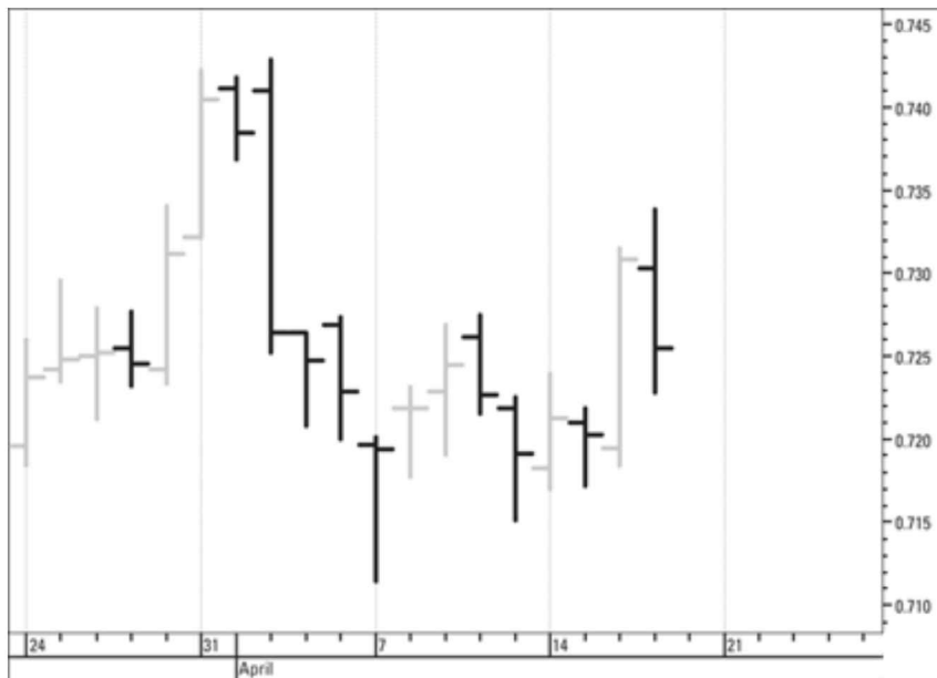
Figure 6-6: Nontrending bars.
