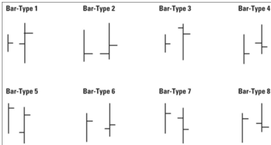
Figure 6-7: Fitschen's simple bar-scoring.
