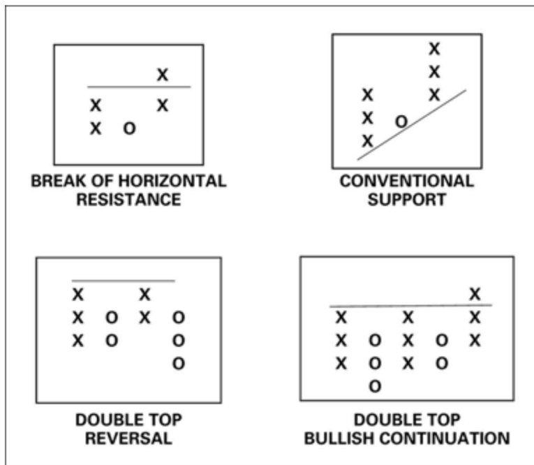
Figure 15-2: Patterns on point-and-figure charts.
