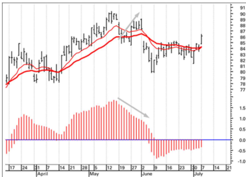
Figure 12-8: MACD histogram.
