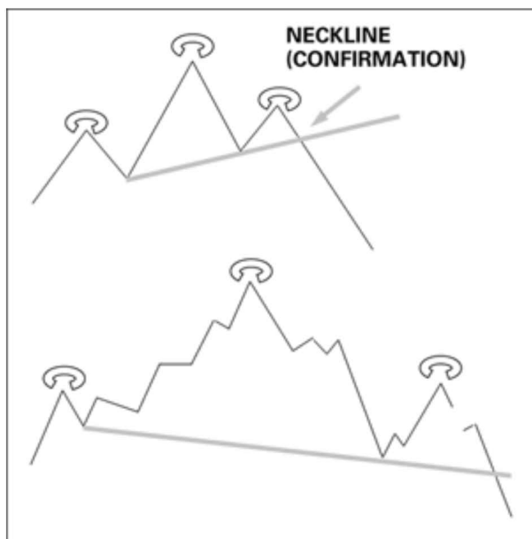
Figure 9-6: Head-and-shoulders patterns.
