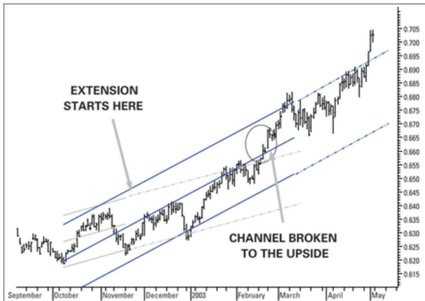
Figure 11-6: Two standard error channels.
