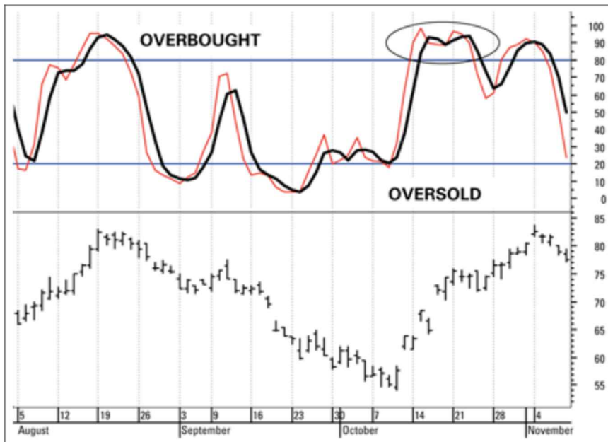
Figure 13-4: Stochastic oscillator.
