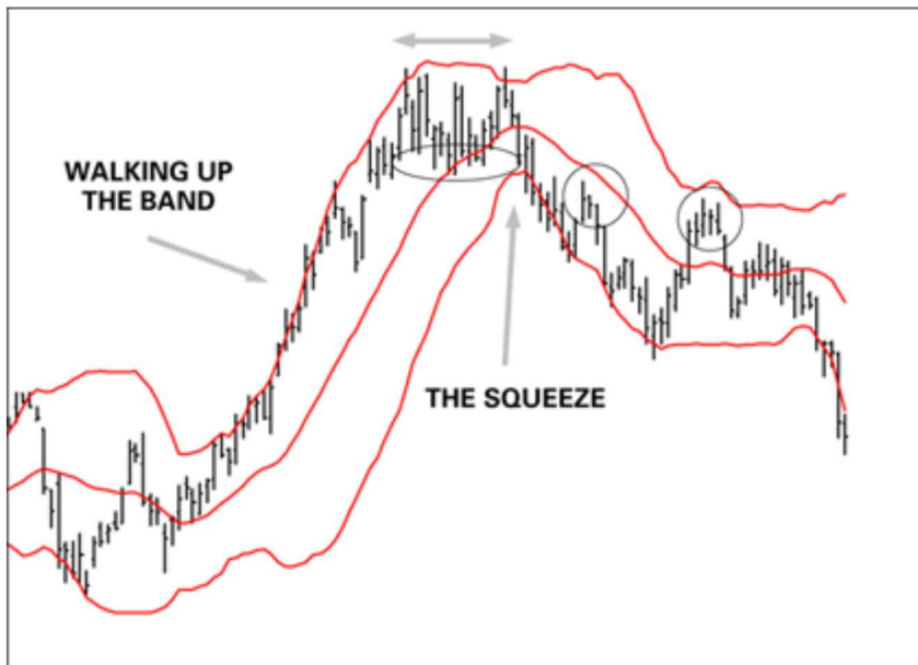
Figure 14-5: Bollinger bands.
