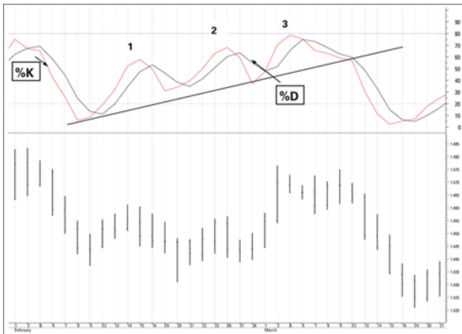
Figure 13-5: Bullish divergence.
